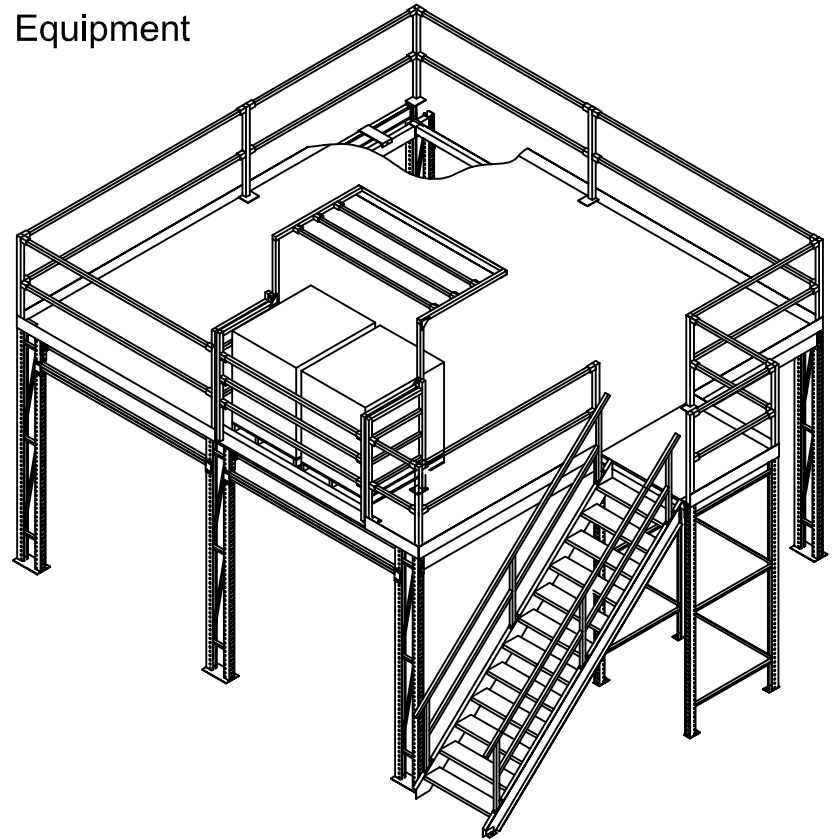
Q-rack mid-span, full-mat storage platform with double spring gate.
