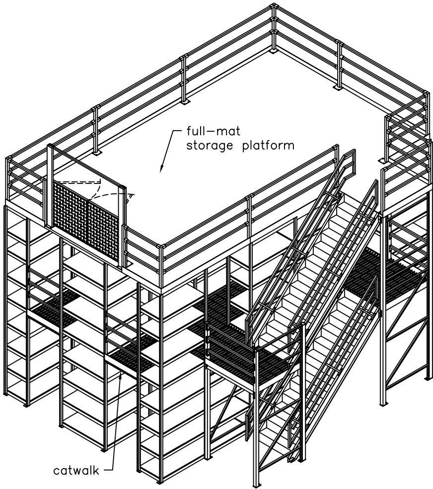
Double high Q-shelf storage system with catwalks. Third level full-mat storage platform including pallet drop using spring gate.
