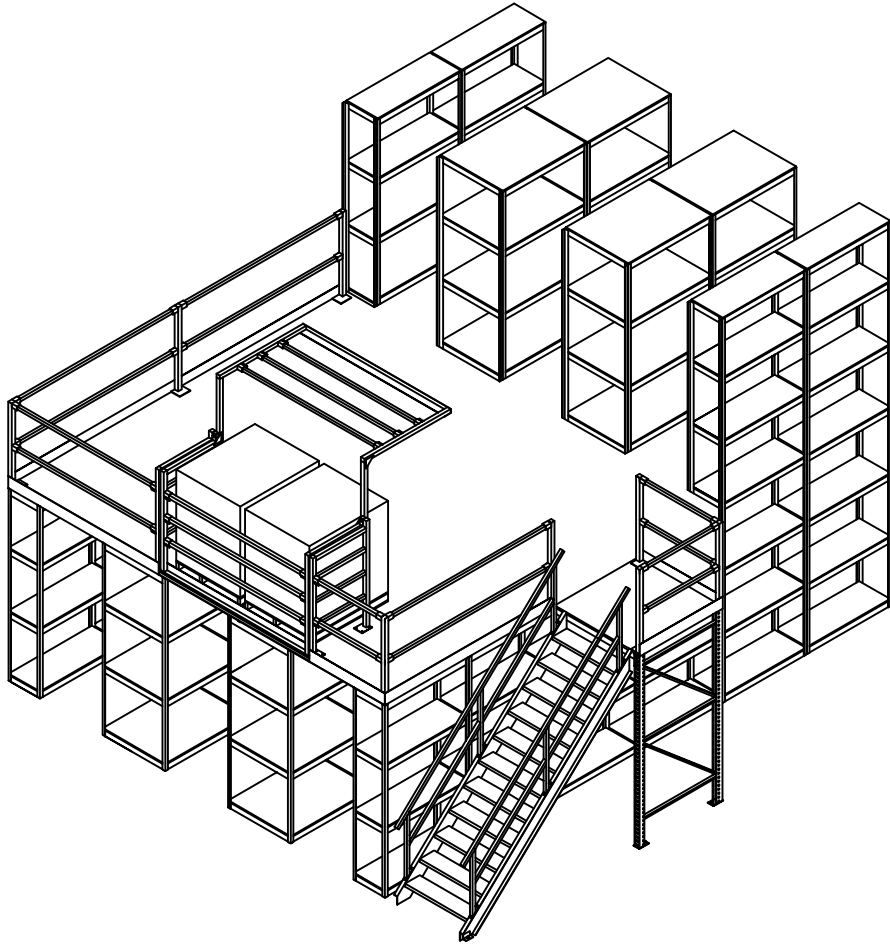
Combination Q-shelf double high storage system with catwalks. Includes shelf supported full-mat storage / staging area.
