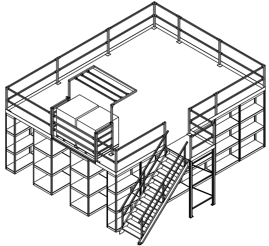
Q-shelf supported full-mat storage platform with double spring gate
